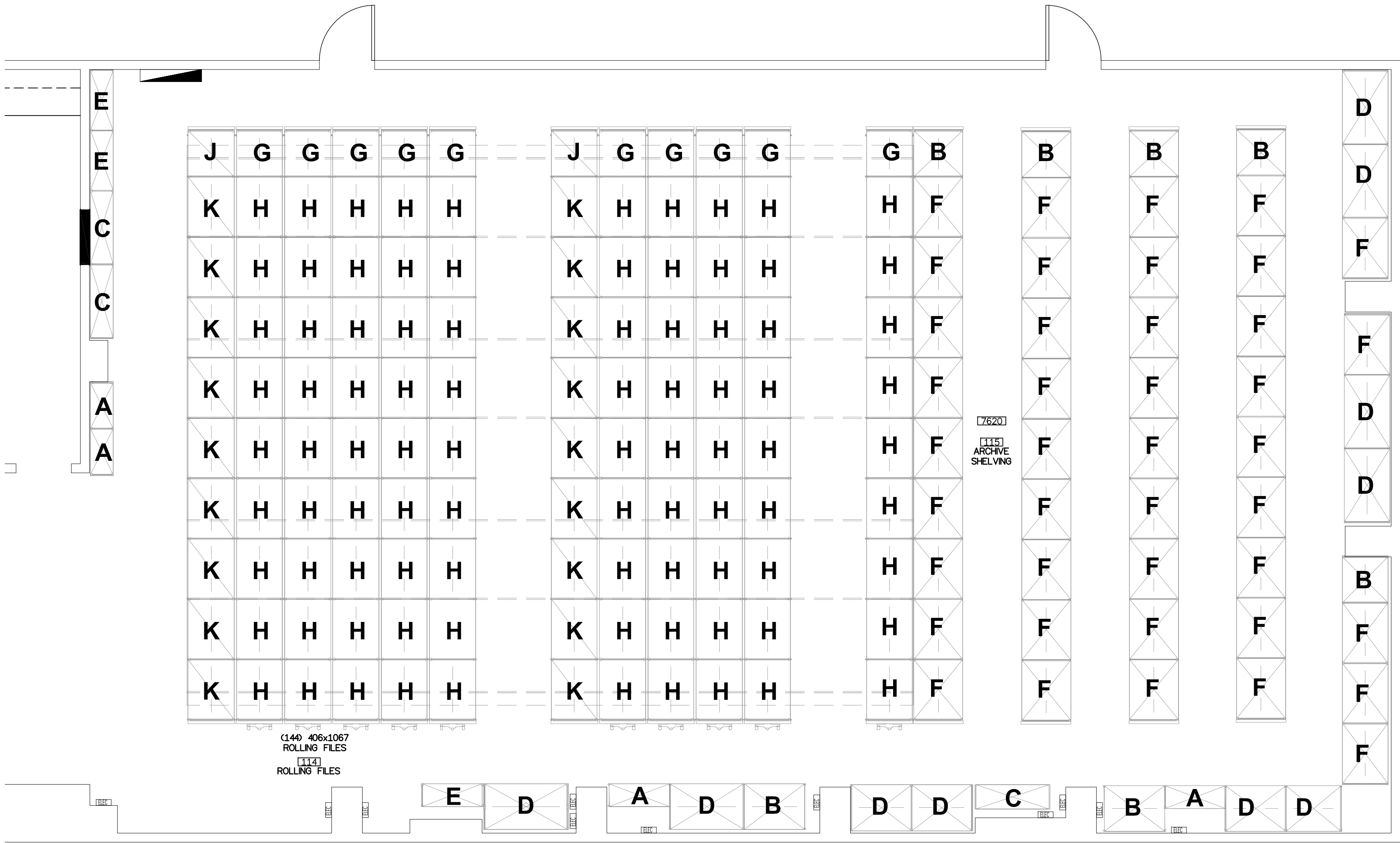
1 PARTIAL FLOOR PLAN - SHELVING LAYOUT A1 A1 1:50
