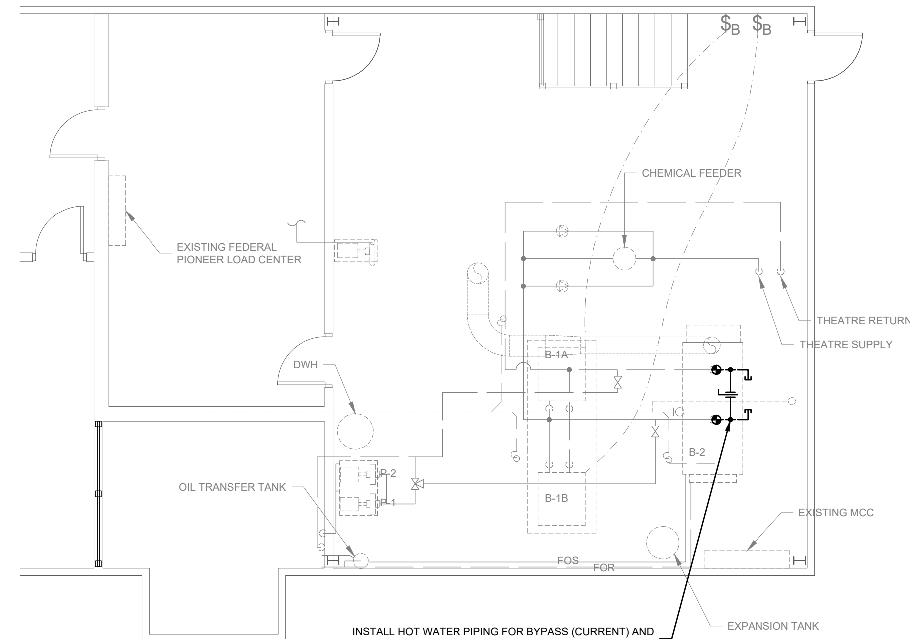
6 PENTHOUSE - NEW HEATING LAYOUT (PHASE 4)
