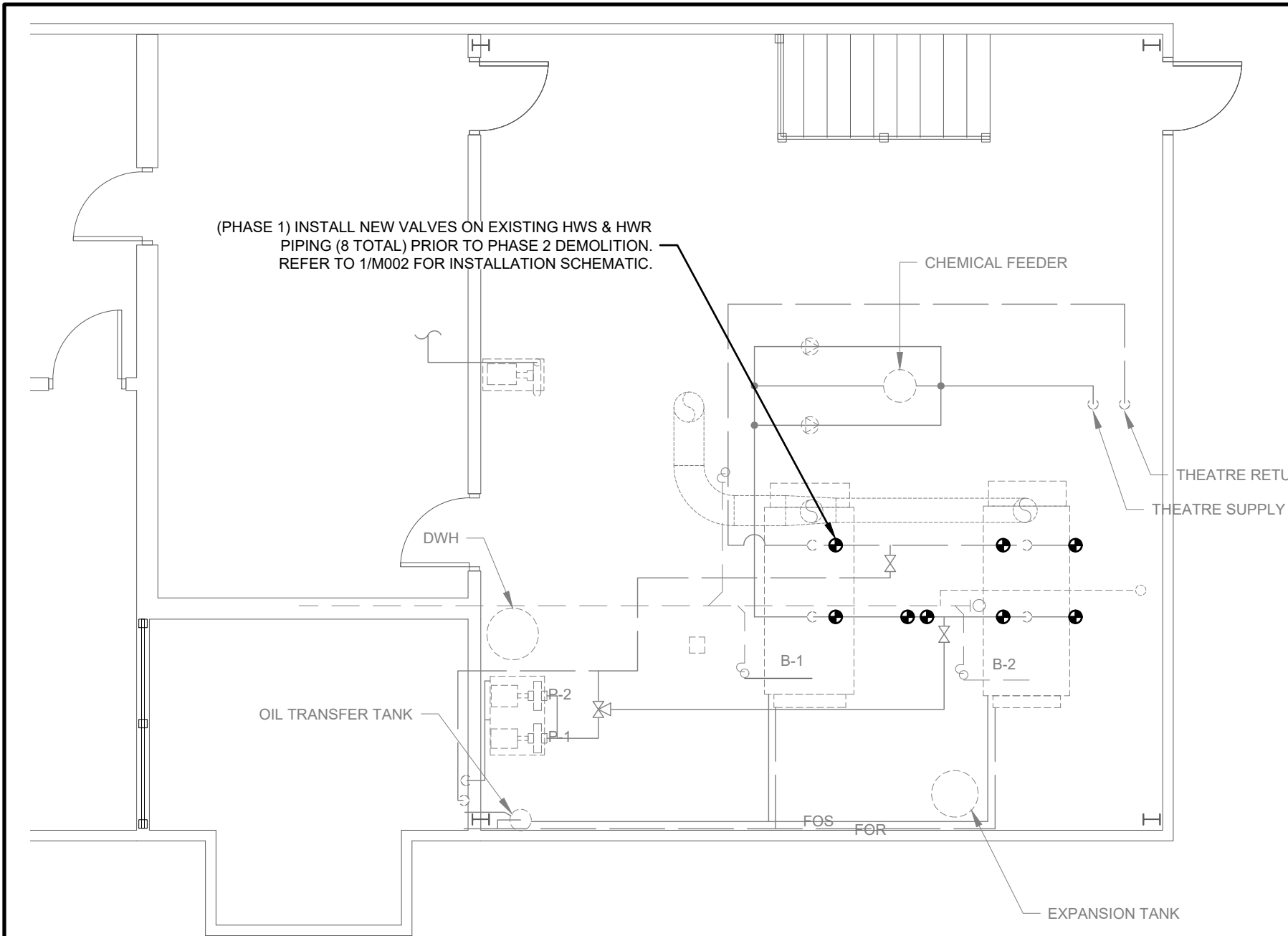
1 PENTHOUSE - NEW HEATING LAYOUT (PHASE 1)
