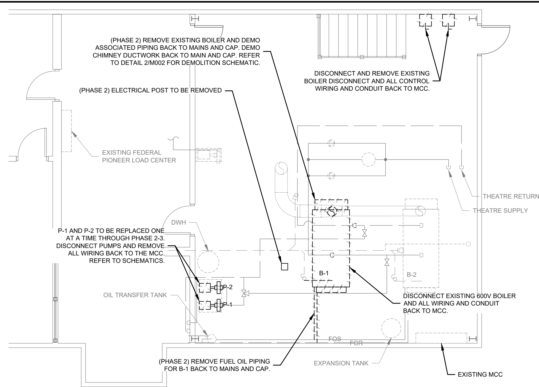
2 PENTHOUSE - DEMOLITION LAYOUT (PHASE 2)
