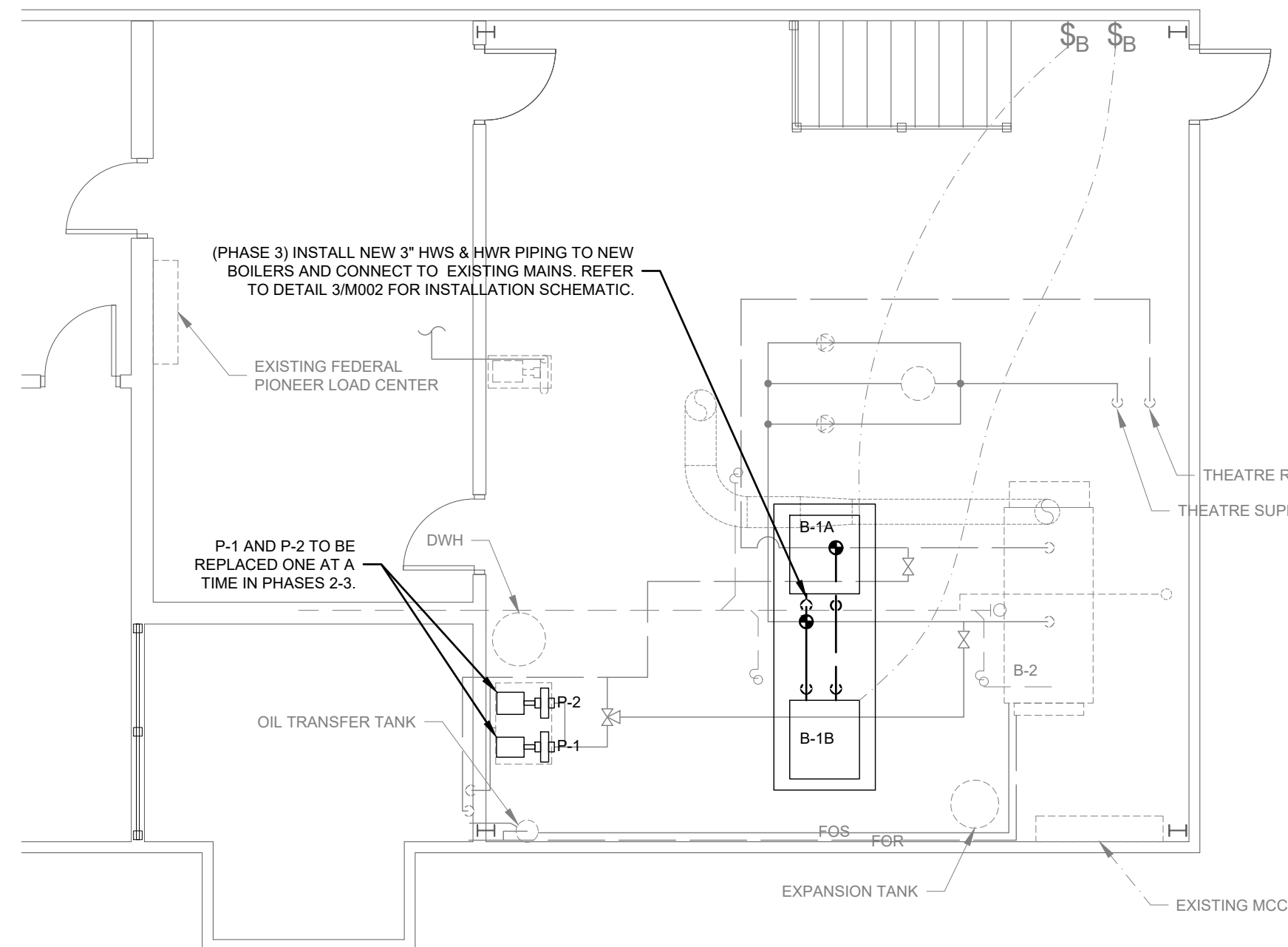
5 PENTHOUSE - NEW HEATING LAYOUT (PHASE 3)
