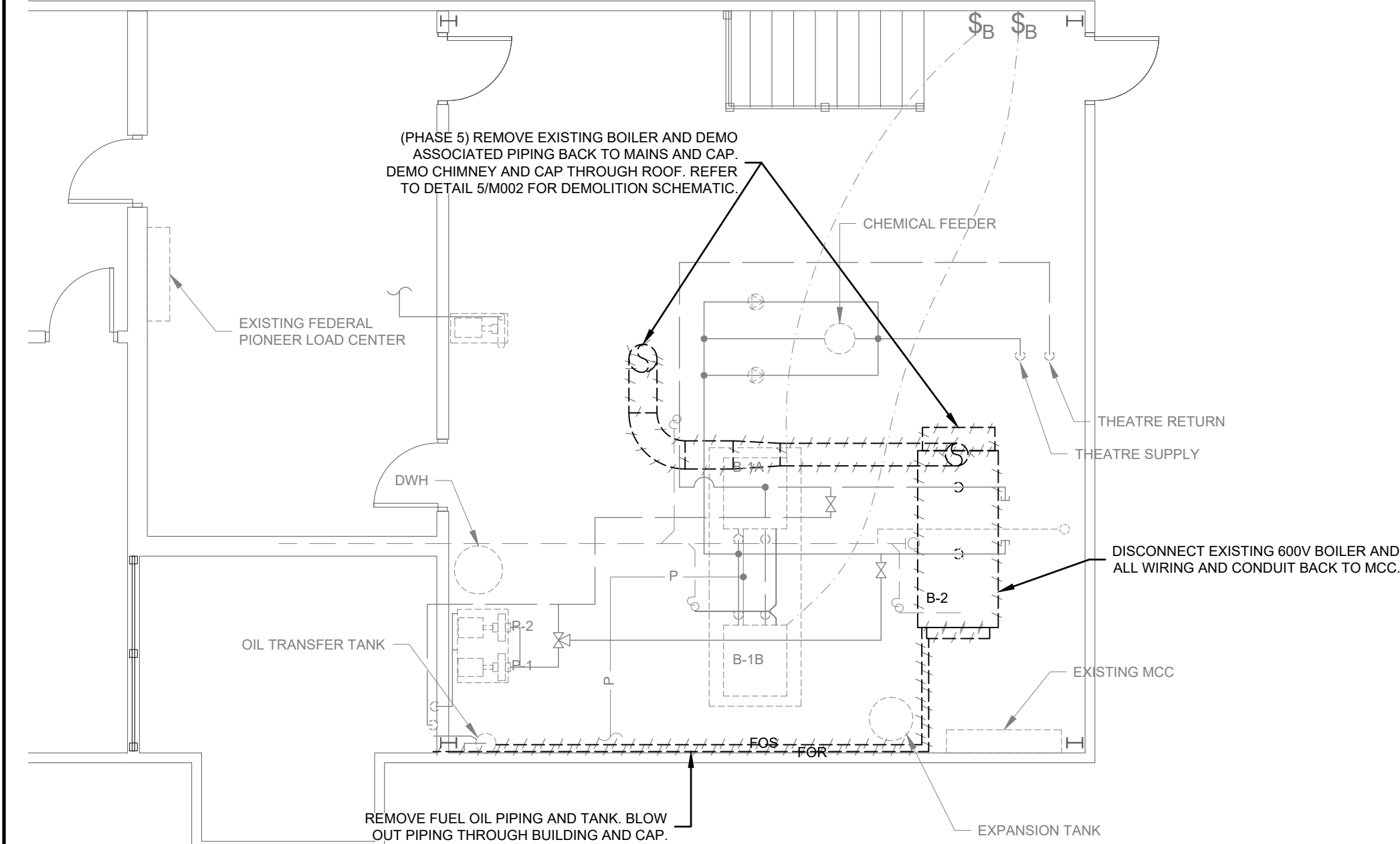
7 PENTHOUSE - DEMOLITION LAYOUT (PHASE 5)
