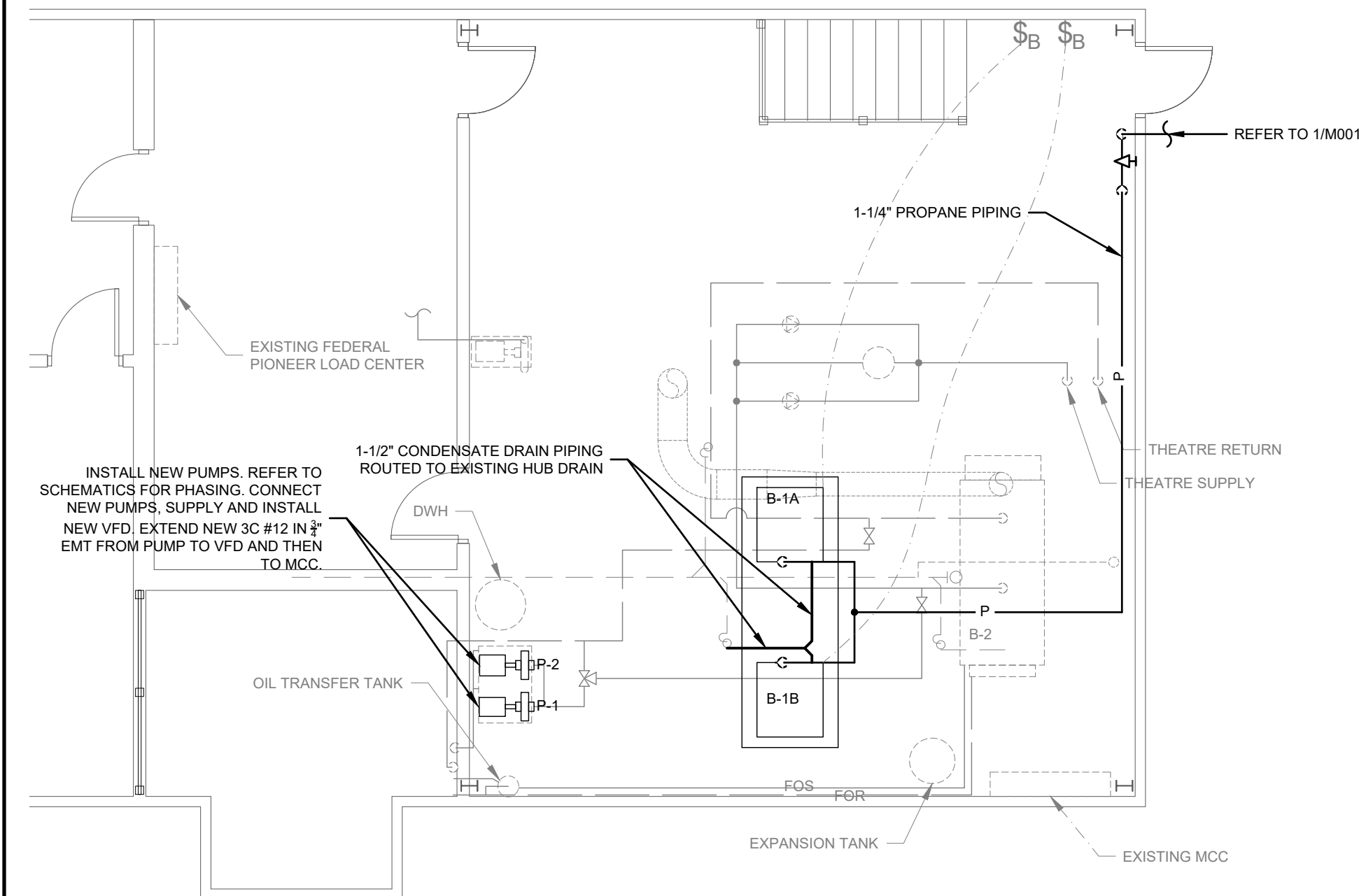
4 PENTHOUSE - NEW PLUMBING LAYOUT (PHASE 3)
