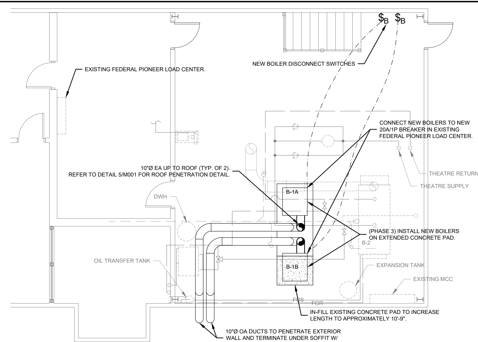
3 PENTHOUSE - NEW VENTILATION LAYOUT (PHASE 3)
